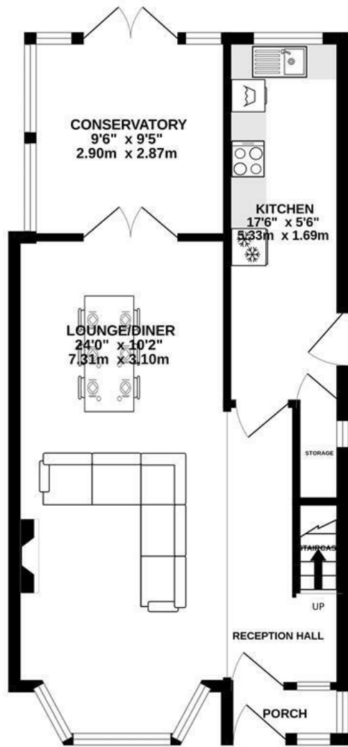
GROUND FLOOR 507 sq.ft. (47.1 sq.m.) approx.
